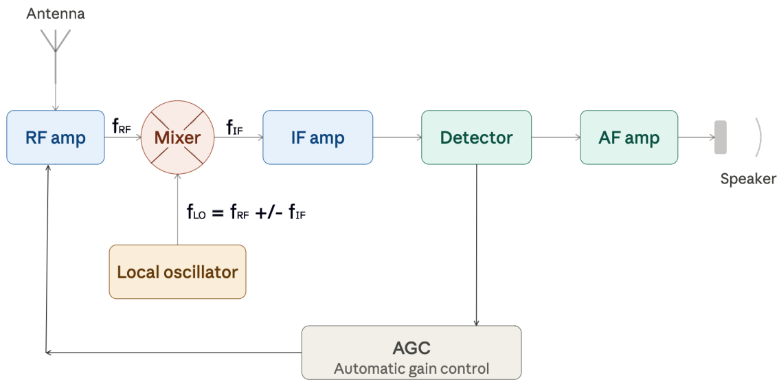
Figure 7-1. A block diagram of a superheterodyne receiver.
