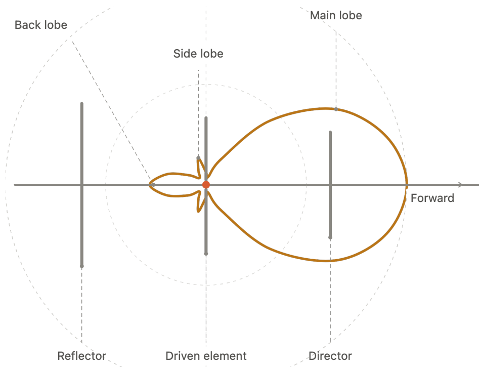
Figure 4-2. As the radiation pattern above shows, a Yagi antenna concentrates signals in one direction.
