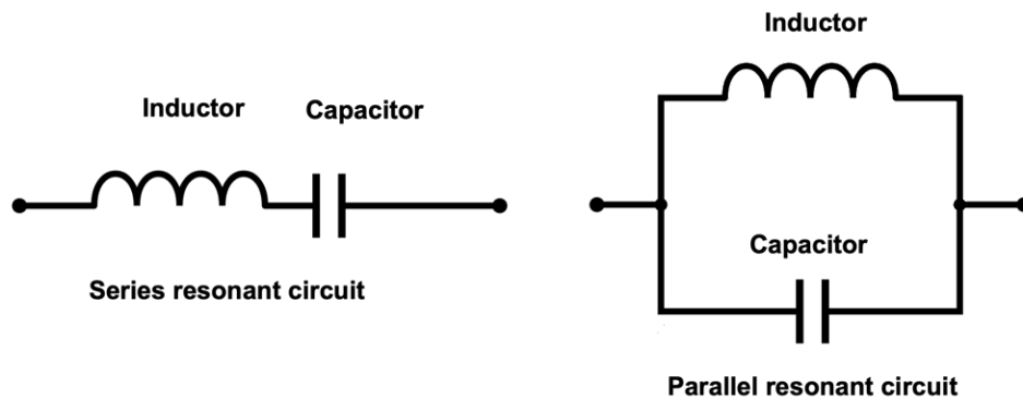
Figure 2-6. A resonant or tuned circuit consists of an inductor and a capacitor connected in series or in parallel.
